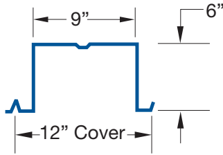
Type "H" Deck Available in acoustical
