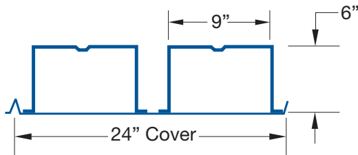
Type "H-Cell" Deck Available in acoustical
