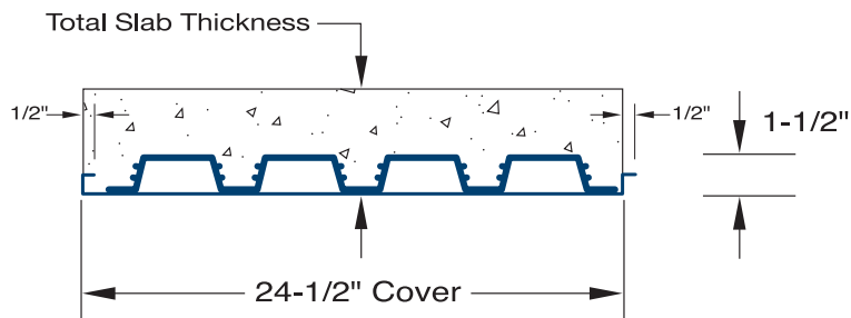
Type 1-1/2" Composite Cellular Acoustical Type Shown
